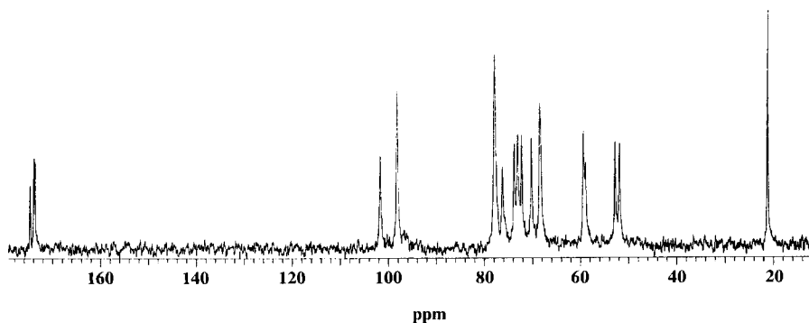
Fig. 1. 13 C NMR spectrum of O-deacetylated HMW H13.
